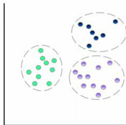
Clustered Data
